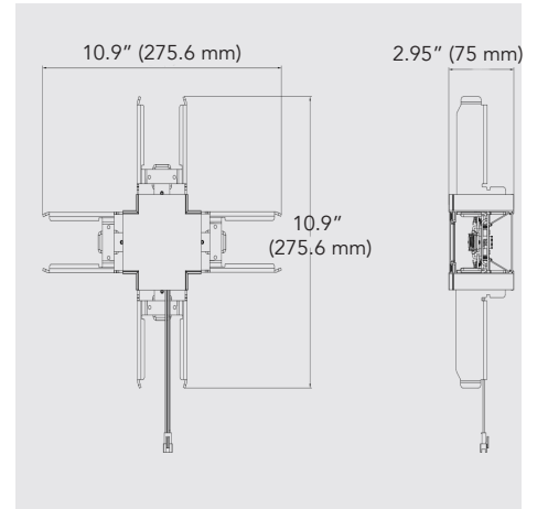
"X" Connector
