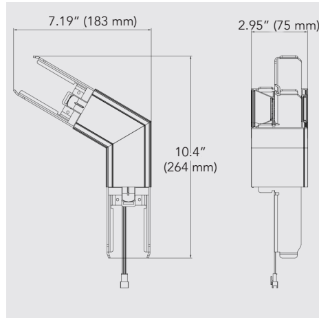
"V" Connector
