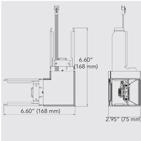
"L" Connector
