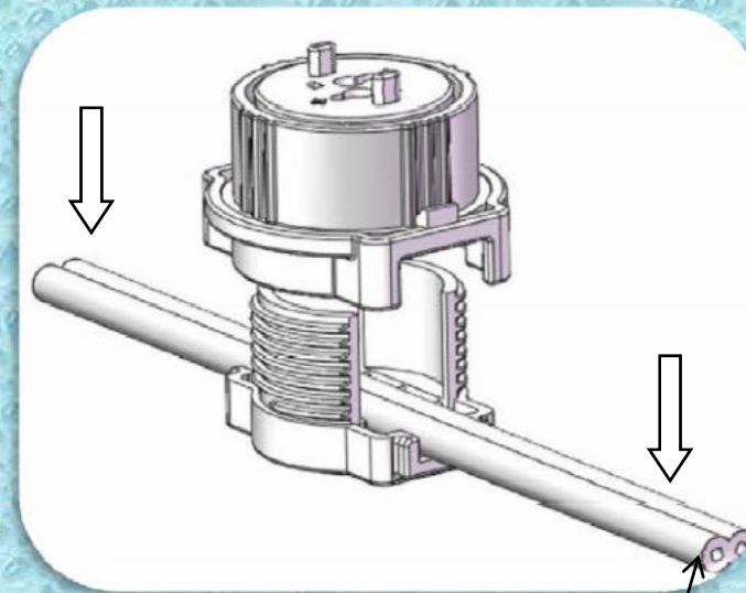
Underground Cable
