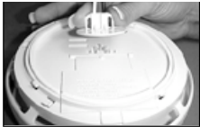
FIGURE 2 ATTACHING THE AC QUICK-CONNECT WIRE HARNESS
