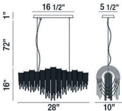
Draped nickel chain wrapped around curved nickel strips
